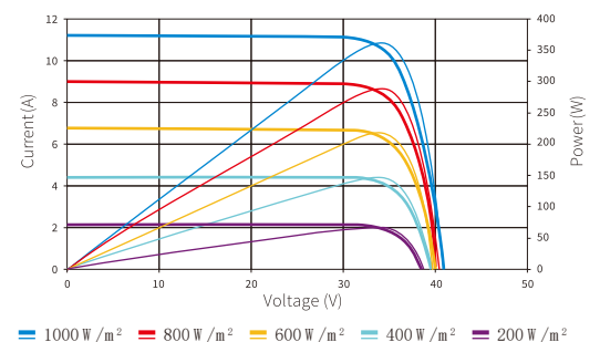
Current-Voltage & Power-Voltage Curve (395)
